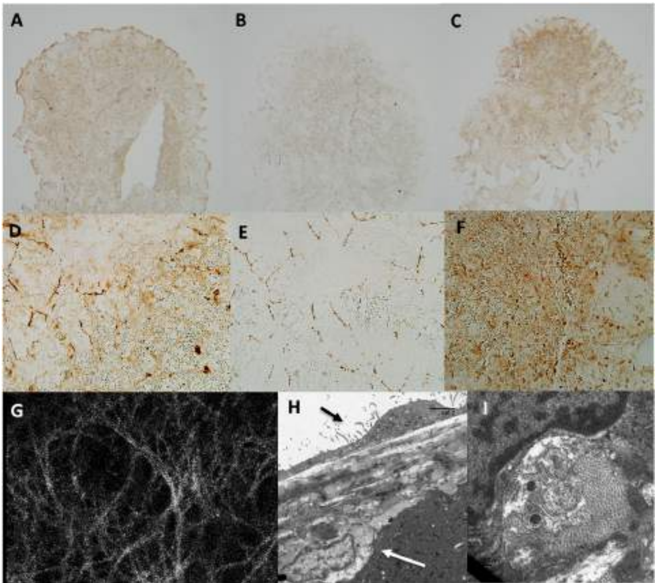
FIGURE 10. Dense network of acetylcholine esterase–positive nerves immediately below the splenic capsule. ( A and D ) Thin (5 \mu\text{m} ) sections through the frontal plane of the splenic capsule indicate strong and diffuse positive staining for the pan-neuronal marker PGP9.5 in the capsular layer. ( A ) Original magnification \times 5 . ( D ) Original magnification \times 20 . ( B and E ) Thin (5 \mu\text{m} ) sections through the frontal plane of the splenic capsule indicate strong positive staining for the sympathetic neuronal marker tyrosine hydroxylase in the capsular layer, with tyrosine hydroxylase–positive tissue forming a loose web of interconnected nerves. ( B ) Original magnification \times 5 . ( E ) Original magnification \times 20 . ( C and F ) Thin (5 \mu\text{m} ) sections through the frontal plane of the splenic capsule indicate strong and diffuse positive staining for the parasympathetic neuronal marker acetylcholine esterase in the capsular layer. ( C ) Original magnification \times 5 . ( F ) Original magnification \times 20 . ( G ) The splenic capsule viewed at 40\times on a confocal microscope. Tissue was loaded with the \text{Ca}^{2+} -sensitive indicator fluo-4. Note a dense layer of nerve tissue can be observed directly below the mesothelial cell layer across the entire splenic capsule. The density of this neural web is much greater than that observed in ( B ) and ( E ) in tissue stained positive for tyrosine hydroxylase, indicating additional nerve tissue is present. Activation of these nerves can be stimulated by electrical field stimulation (see supplement). ( H ) Transmission electron microscopy indicates that nerves sit directly below the splenic capsule. Black arrow indicates capsular mesothelial cell. White arrow indicates nerve closely associated with the splenic capsule. Bar, 5 \mu\text{m} . ( I ) Nerves are identified by the presence of intracellular vesicles typical of synaptic junctions.
