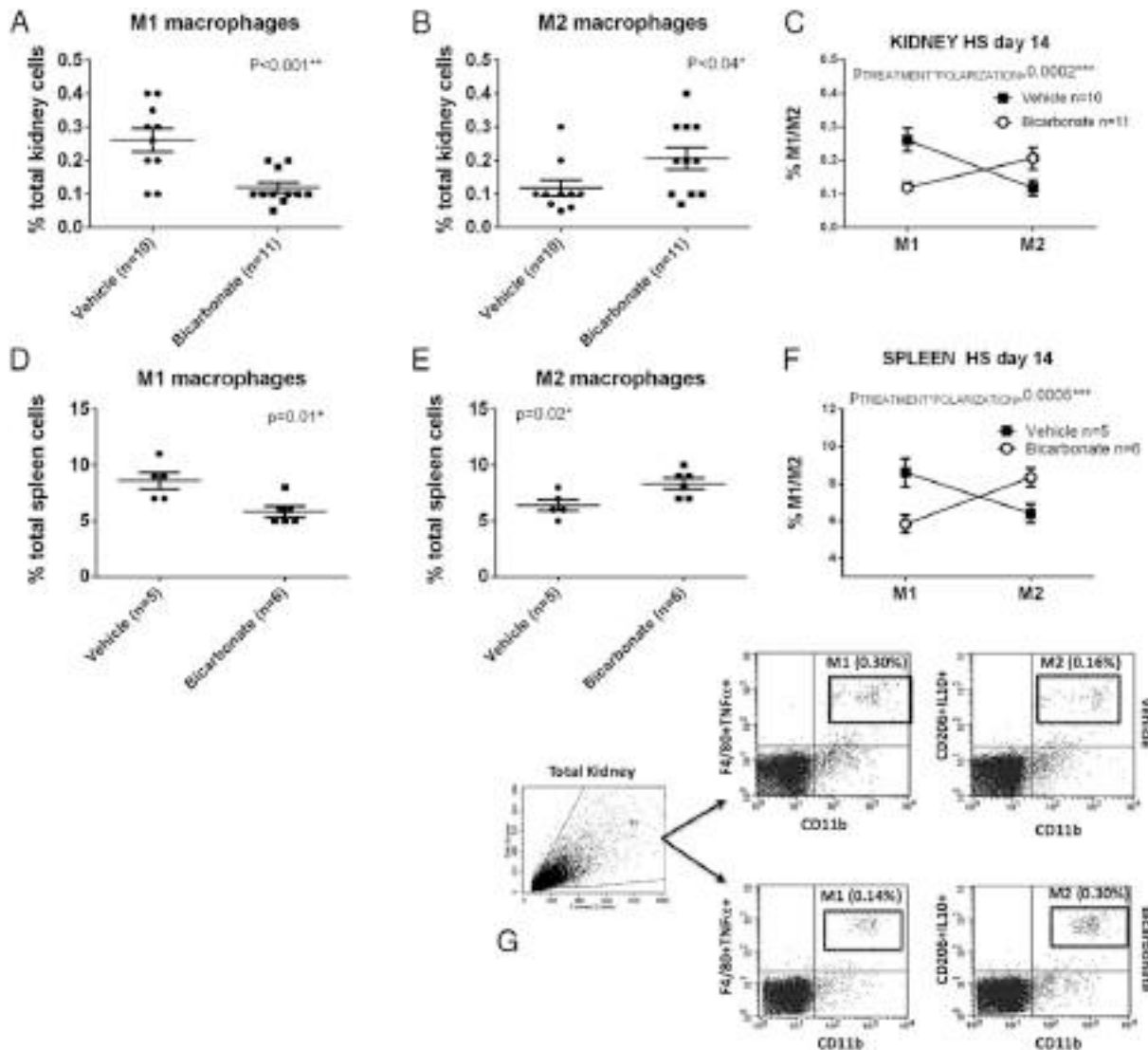
FIGURE 1. Data from flow cytometric analysis of macrophage polarization (M1/M2) from kidneys and spleen from male Dahl SS rats drinking 0.1 M NaHCO 3 (bicarbonate) or equimolar NaCl (vehicle) are presented in (A)–(G). All data are from rats placed on treated water (vehicle or bicarbonate) for 3 d before being switched to an HS diet for 14 d prior to tissue harvest. (A) The percentage of total kidney cells identified as M1 macrophages (CD11b/F4/80 + /TNF- \alpha + cells) in vehicle- ( n = 10 ; filled circles) and bicarbonate- ( n = 11 ; filled squares) treated rats. (B) The percentage of total kidney cells identified as M2 macrophages (CD11b/CD206 + /IL10 + cells) in vehicle- ( n = 10 ; filled circles) and bicarbonate- ( n = 11 ; filled squares) treated rats. (C) Relative expression of M1 and M2 macrophages expressed as a percentage of total kidney cells in vehicle- (filled squares) and bicarbonate- (open circles) treated rats. (D) The percentage of total spleen cells identified as M1 macrophages (CD11b/F4/80 + /TNF- \alpha + cells) in vehicle- ( n = 10 ; filled circles) and bicarbonate- ( n = 11 ; filled squares) treated rats. (E) The percentage of total spleen cells identified as M2 macrophages (CD11b/CD206 + /IL10 + cells) in vehicle- ( n = 10 ; filled circles) and bicarbonate- ( n = 11 ; filled squares) treated rats. (F) Relative expression of M1 and M2 macrophages expressed as percentage of total spleen cells in vehicle- (filled squares) and bicarbonate- (open circles) treated rats. (G) Representative gating images from kidneys of HS-treated rats.
